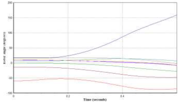
Fig. 8: Rotor angle trajectories for an unstable condition (Case 4)
