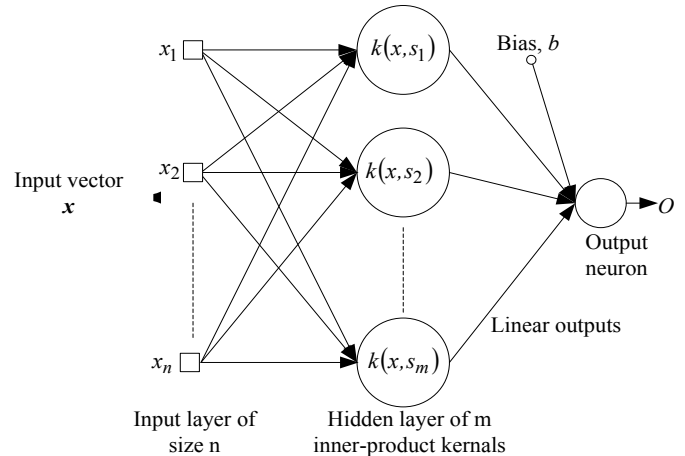
Fig. 2: General architecture of support vector machine
