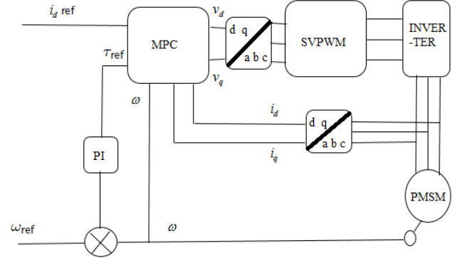
Fig. 1. Proposed MPC-SVPWM fed PMSM drive
