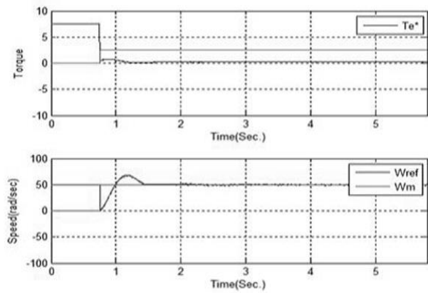
Fig.6. Speed and Torque vs Time
