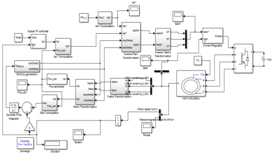
Fig.3. Realization of Indirect Rotor Field Oriented Control algorithm using Matlab/Simulink
