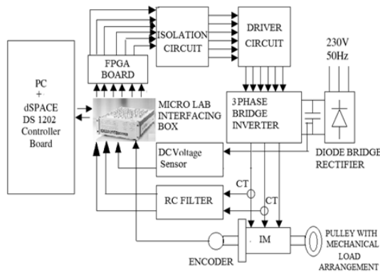
Fig.4. Hardware Configuration
