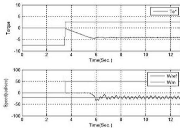
Fig. 16. Reference and Estimated Speed, Torque vs Time
