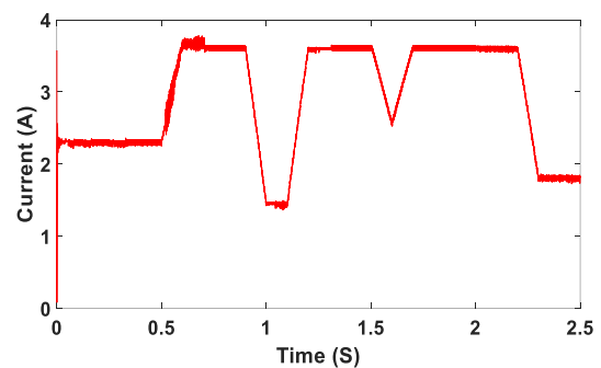
Fig. 20. Output Simulation of Battery Current under FCE
