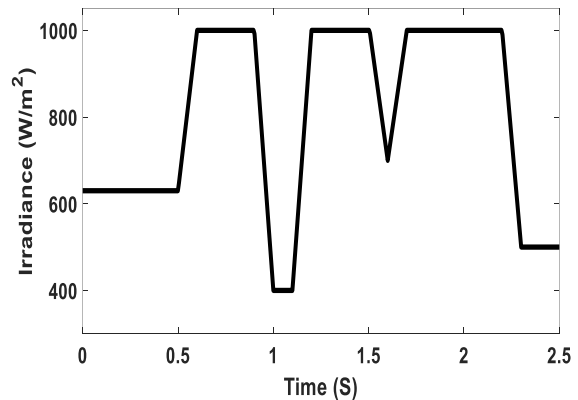
Fig. 9. Simulated Irradiance Levels Waveform under FEC
