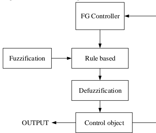
Fig 4: FUZZY-GENETIC Controller
