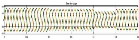
Fig 10: Generated voltage
