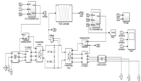
Fig 9: Simulation model for UPQC with FG controller
