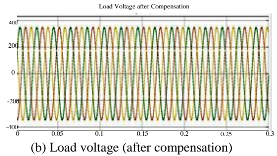
Fig 8: Performance of DVR
