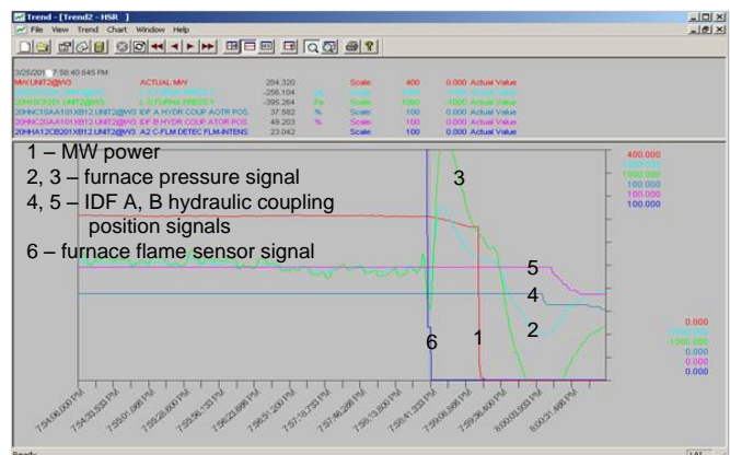
Fig. 1. Effects of the furnace pressure oscillation
