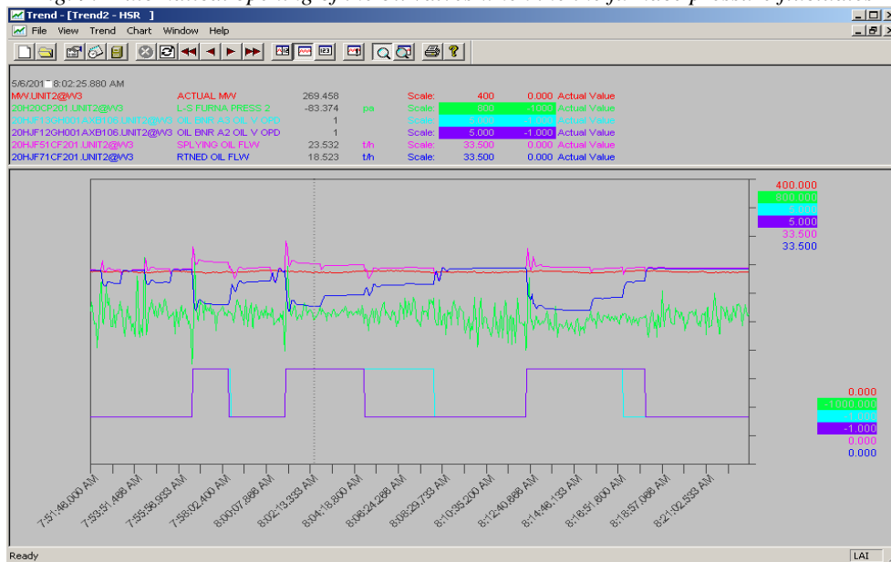
Fig. 9. Automatical opening of the oil valves when the the furnace pressure fluctuates
