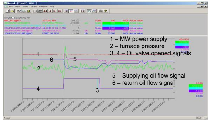
Fig. 7. Automatical opening of the oil valves when the furnace pressure is less than -250pa
