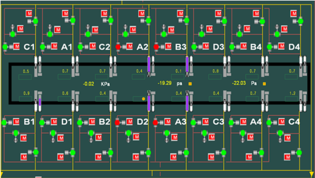
Fig. 3. Test of the oil burner start sequence by manual mode
