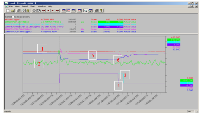
Fig. 8. Automatical opening of the oil valves when the furnace pressure more than +250pa
