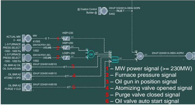
Fig. 5. Improvement of the oil valve logic for the oil valve in automatic opening
