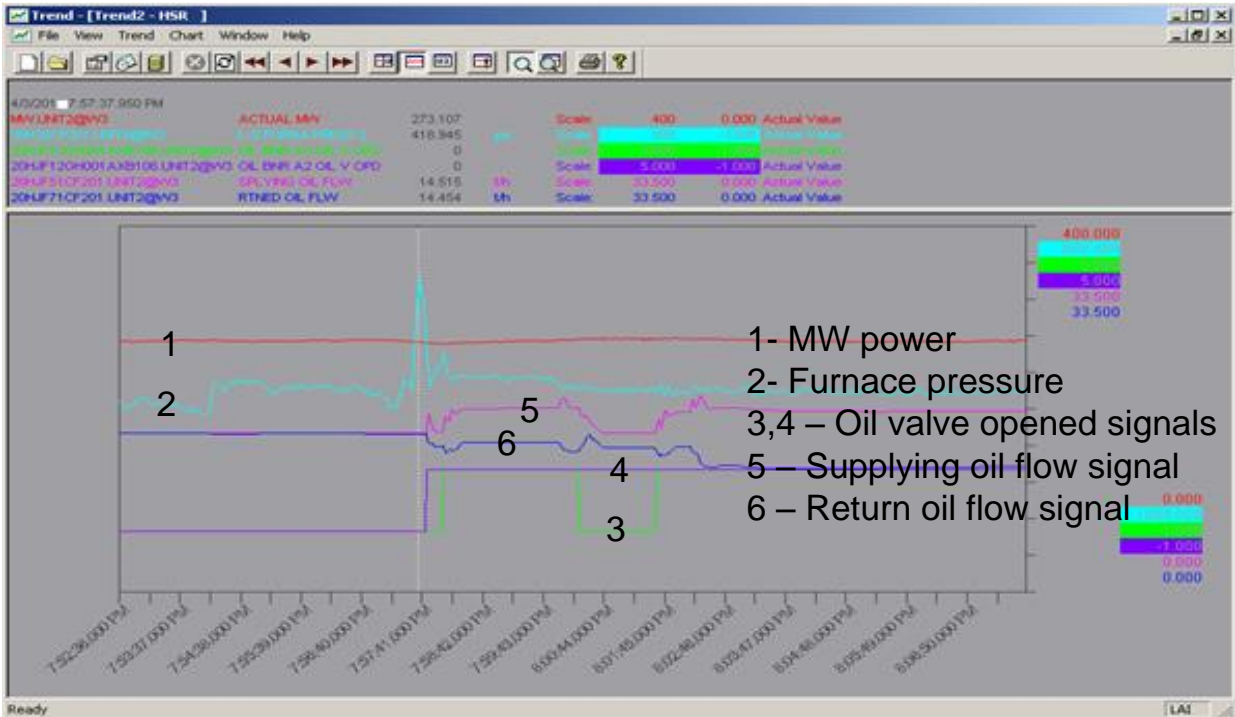
Fig. 4. Results for opening of the oil angle valve by manual mode
