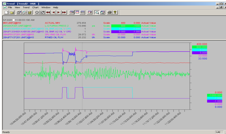
Fig. 9. Automatical opening of the oil valves when the the furnace pressure fluctuates
