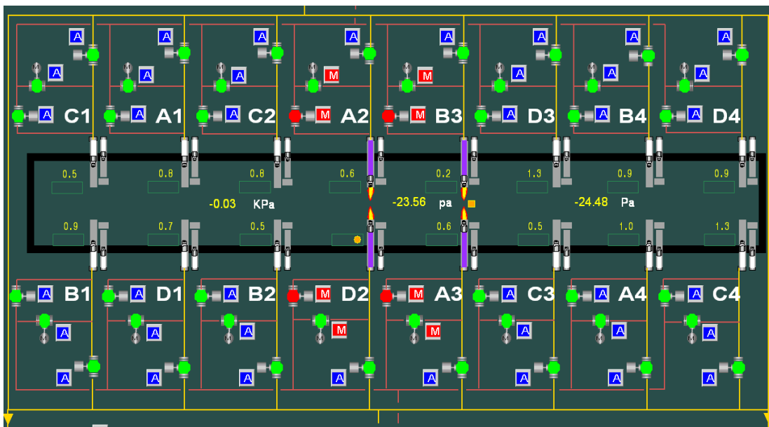
Fig. 6. Oil valves are taken into automatical mode
