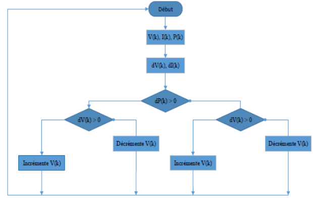
Fig. 3. Perturb and Observe Algorithm
