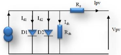
Fig. 1. Equivalent Circuit of a Solar Cell
