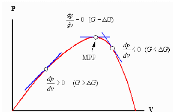
Fig. 2. Power Versus Voltage for Perturb and Observe Algorithm [6]
