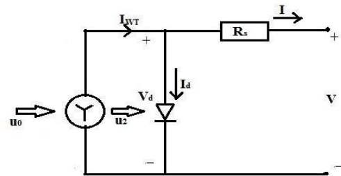
Fig.4. Equivalent circuit of wind turbine
