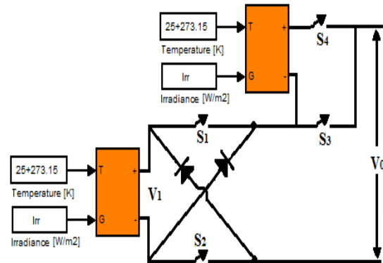
Fig. 9. Proposed inverter with two voltage sources.
