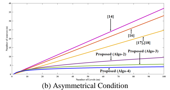
Fig. 6. Levels vs Sources
