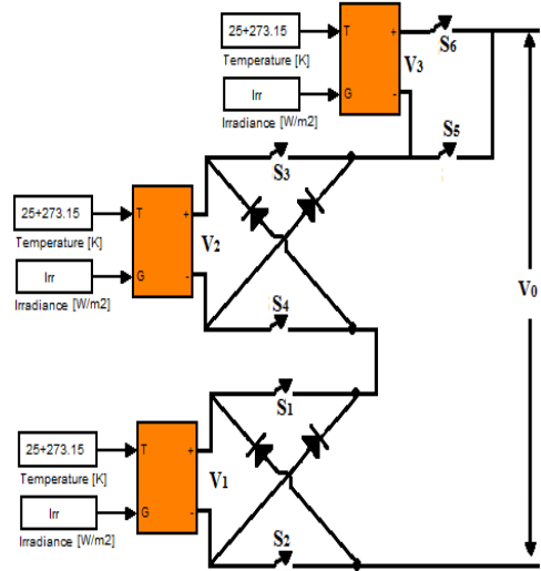
Fig.12. Proposed inverter with three voltage sources.
