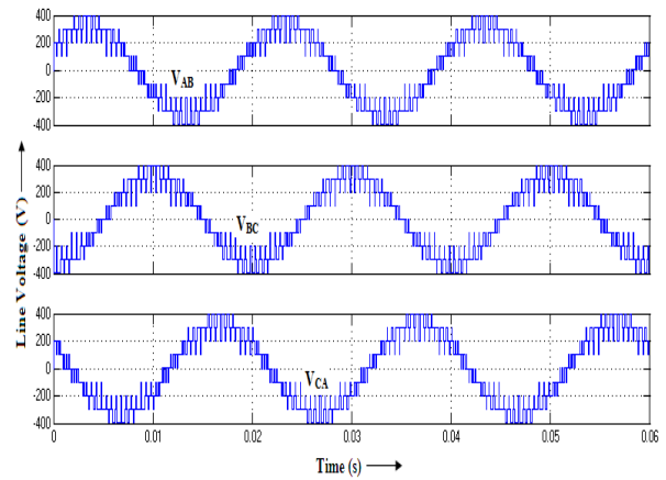
Fig.9 Line voltage waveform
