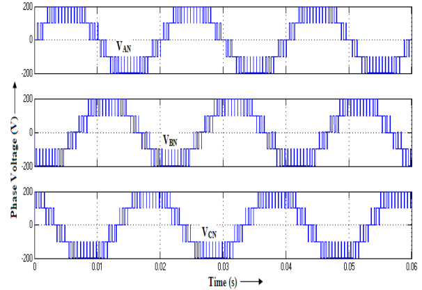
Fig. 8 Phase voltage waveform
