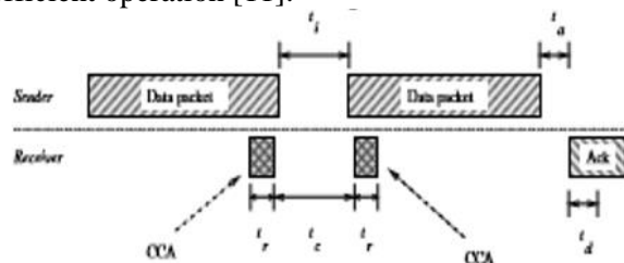
Fig . 11. ContikiMAC transmission and CCA timing.
