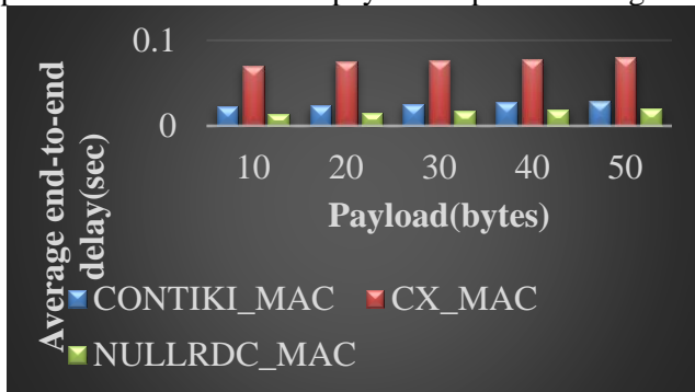
Fig. 20. Average end-to-end delay offered by notes for three different MACs with payload varied from 10 to 50 bytes
