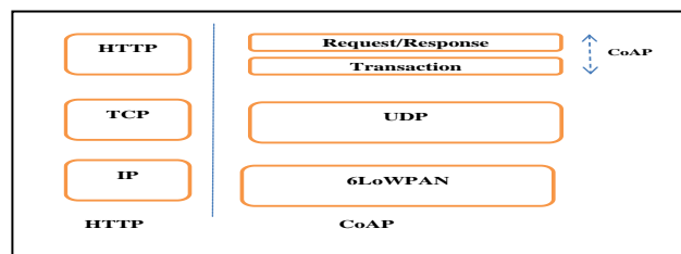
Fig. 6. HTTP and CoAP stack comparison
