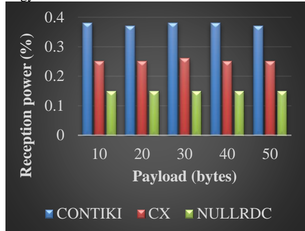
Fig. 22. Reception power consumed by notes for variations in payload
