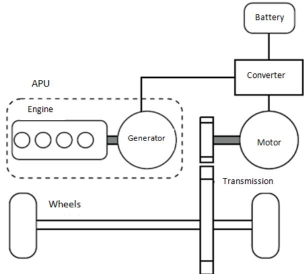
Fig.8 Hybrid Architecture
