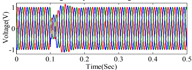
Fig.12 Load Voltage
