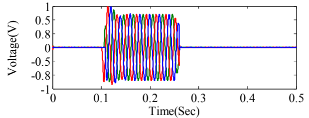
Fig.14 Injection Voltage
