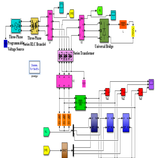
Fig.9 Simulation Diagram of DVR Based 7-level H bridge multilevel inverter
