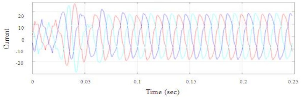
Fig.11 Waveform for source voltage and current (PI controller)
