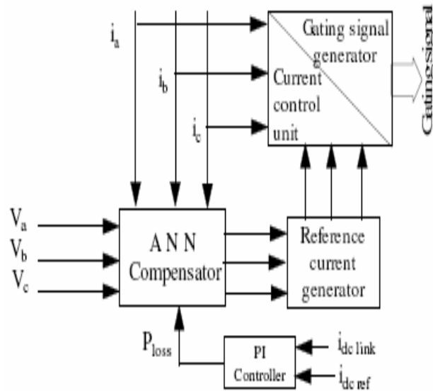
Fig. 6. Block diagram of ANN-based system
