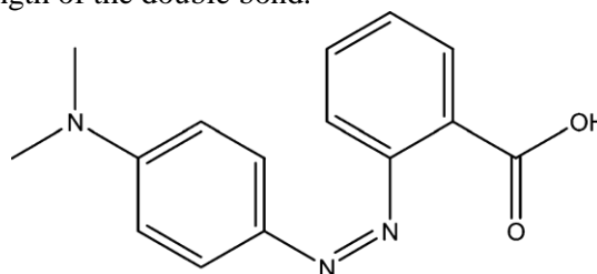
Fig. 1. Azo bond structure in colour compounds
