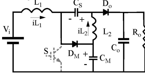
Fig.3.First operation stage
