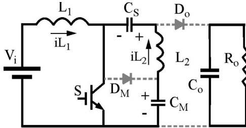
Fig.4.Second operation stage
