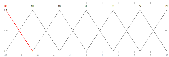
Fig.6. Membership functions of inputs E and EC
