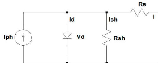
Fig.1.Schematic diagram of single diode solar cell
