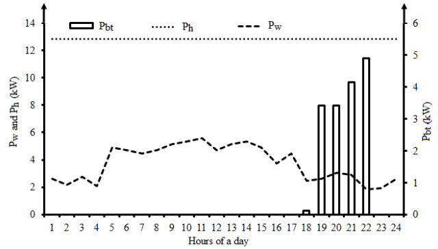
Fig. 9 Real Power generated from different sources using GWO for case 5
