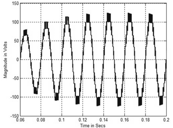
Fig 8. 15level output voltage waveform of proposed MLI with splitting capacitors
