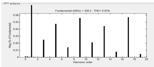
Fig 11 THD plot of output voltage of 15level MLI with SITO DC-DC boost converter
