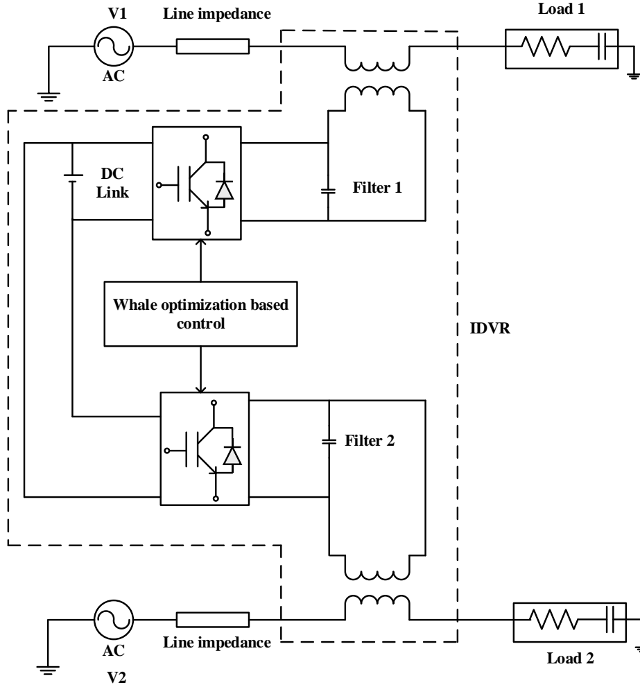
Fig. 3. IDVR between adjacent feeders
