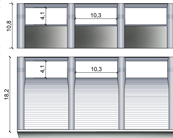
Figure 1.1 Upstream and downstream views of the top discharger
