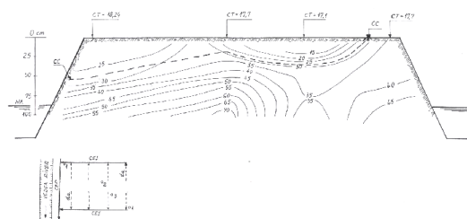
Fig. 4 Chronohydroisopleths – Vedeia watermeadow, left bank, 0-100 cm depth, August
