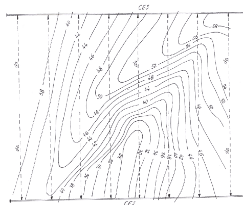
Fig.3 Chronohydroisopleths – Vedeia watermeadow, left bank, 0-100 cm depth, August
