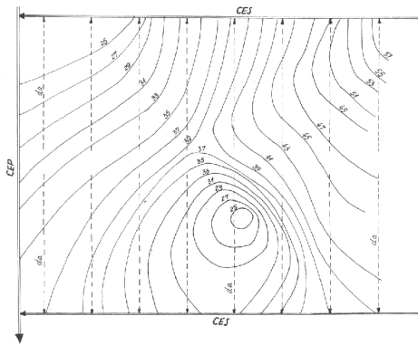
Fig. 1 Chronohydroisopleths – Vedeia watermeadow, left bank, 0-50 cm depth, August
