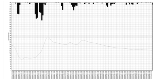
Figure 6 Hydrograph issued by IFAS
