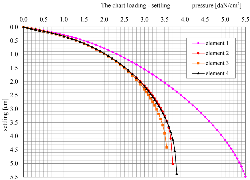
Fig. 2. Loading-settling charts for the elements 1, 2, 3, 4 placed in dug holes
