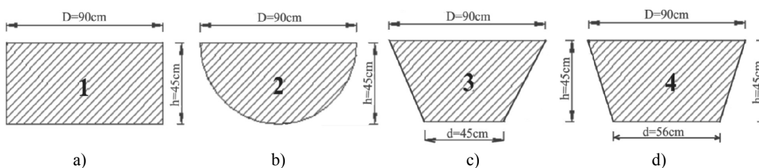
Fig. 1. Types of specially shaped precast elements
