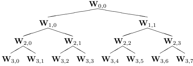
Fig. 1. Wavelet packet decomposition tree down to decomposition level j = 3 .
