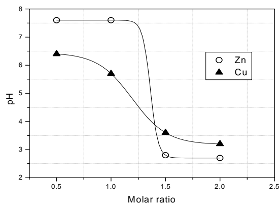
Fig. 1. The mass reaction pH dependence by the molar ratio Me^{2+}: P_2O_7^{4-}
