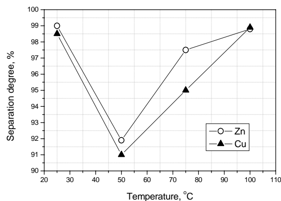
Fig. 6. The zinc and copper separation degree by temperature
