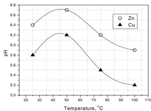
Fig.4. The mass reaction pH dependence by temperature .
