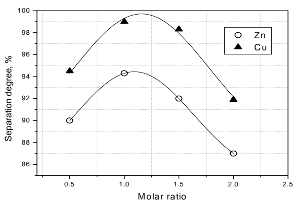
Fig. 3. The zinc and copper separation degree by the molar ratio Me^{2+}: P_2O_7^{4-}
