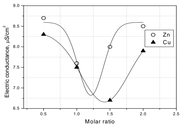
Fig. 2. The electric conductance dependence by the molar ratio Me^{2+}: P_2O_7^{4-}
