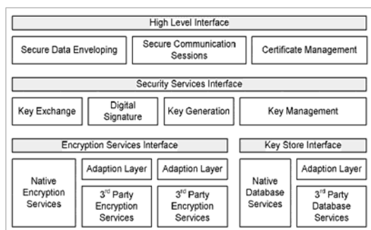
Fig. 1. Cryptlib Architecture Diagram
