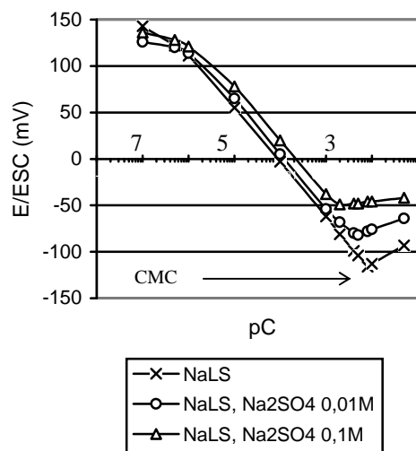
Figure 1. The influence of the ionic strength on the response function of the laurylsulphate sensible electrode:
