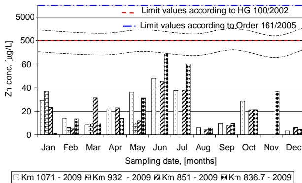
Figure 2. Variation of zinc concentration in Bazias Gruia sector (year 2009)
