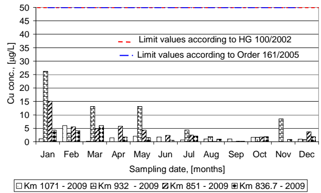
Figure 4. Variation of copper concentration in Bazias Gruia sector (year 2009)
