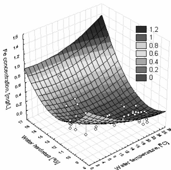
Figure 8 . The variation of iron concentrations depending on water hardness and temperature
