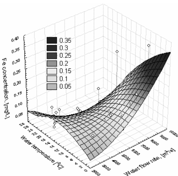
Figure 9. Variation of iron concentrations depending on water temperatures and flow rates
