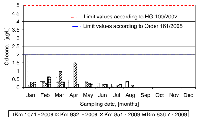
Figure 6. Variation of cadmium concentration in Bazias Gruia sector (year 2009)
