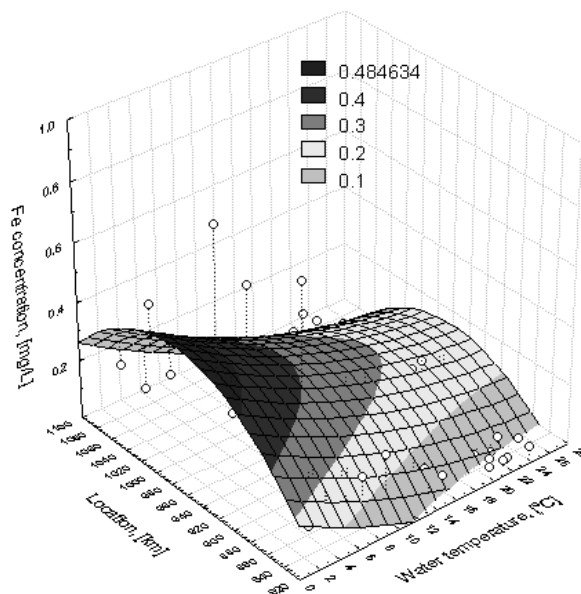
Figure 10. Variation of iron concentrations depending on water temperatures and sampling locations
