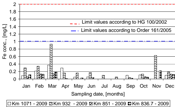
Figure 1. Variation of iron concentration in Bazias Gruia sector (year 2009)
