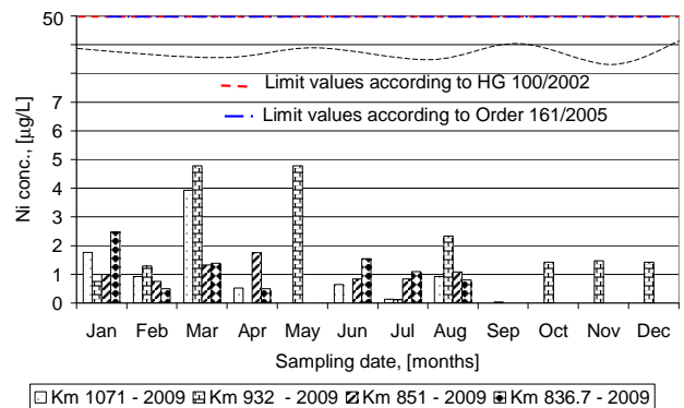
Figure 5. Variation of nickel concentration in Bazias Gruia sector (year 2009)
