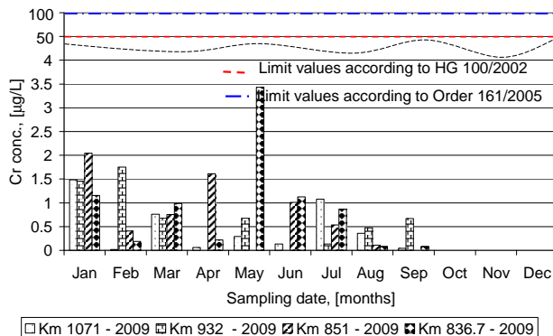
Figure 3. Variation of chrome concentration in Bazias Gruia sector (year 2009)
