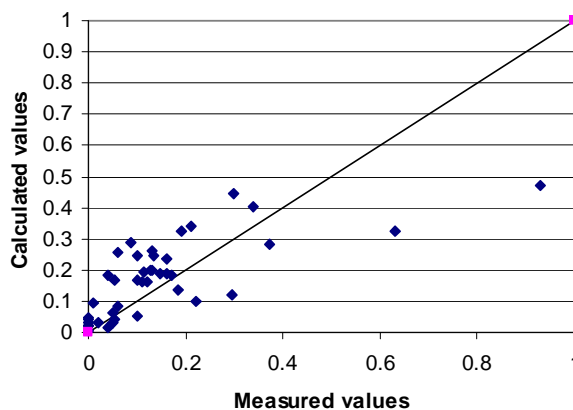
Figure 11. Comparison between the calculated and the measured values of iron concentrations
