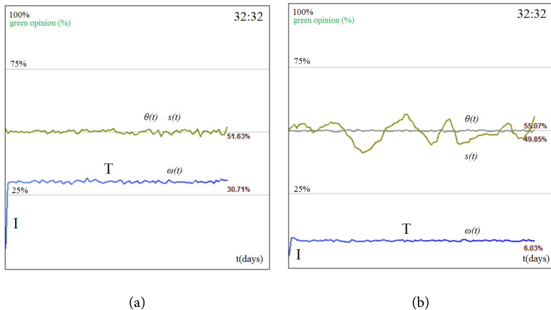
Figure 6.15.: a. Representative simulation depicting opinion evolution in an uncorrelated random scale-free network with 32 red stubborn agents and 32 green stubborn agents: although opinion constantly oscillates, society becomes balanced and stabilizes in the tolerance phase. b. Representative simulation depicting opinion evolution in a random Erdos-Renyi network with 32 red stubborn agents and 32 green stubborn agents. Opinion change is maintained high and opinion presents high oscillations, but the overall state of the society becomes stable and predictable around 50% green opinion.
