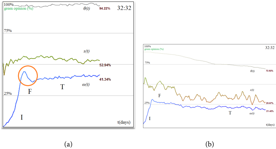
Figure 6.16.: Simulation results for the tolerance-based opinion interaction on a small-world network with 10,000 nodes with 32:32 green-red SAs. a. There are no NullAgents in the population. b. The population consists of 20% randomly placed NullAgents.
