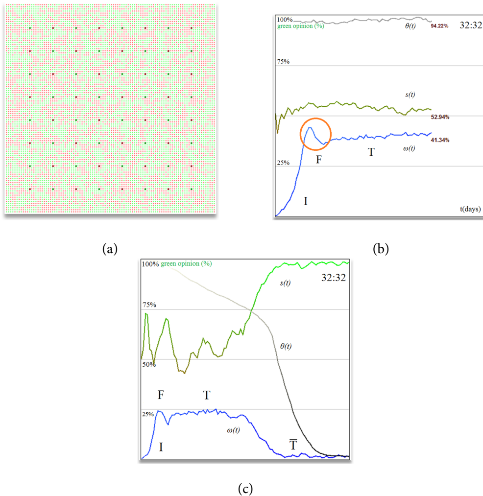
Figure 6.11.: Opinion evolution with homogeneous stubborn agent distribution (32:32) in small-world and scale-free networks. a. Tolerance phase where no visible clusters emerge for small-world networks. b. For small-world networks, social balancing is attained because tolerance remains extremely high ( \theta(t) > 90\% ), opinion change ( \omega ) exhibits the three opinion evolution phases (initiation I , fusion F , and tolerance T ), and never reaches intolerance. The state of the society s(t) is stable. c. Social balancing is not achieved for scale-free networks: tolerance drops constantly and the society reaches the intolerance phase ( \bar{T} ). The state of the society s(t) is unstable during the first three phases of opinion change, then stabilizes as tolerance ( \theta ) and opinion change ( \omega ) fall.
