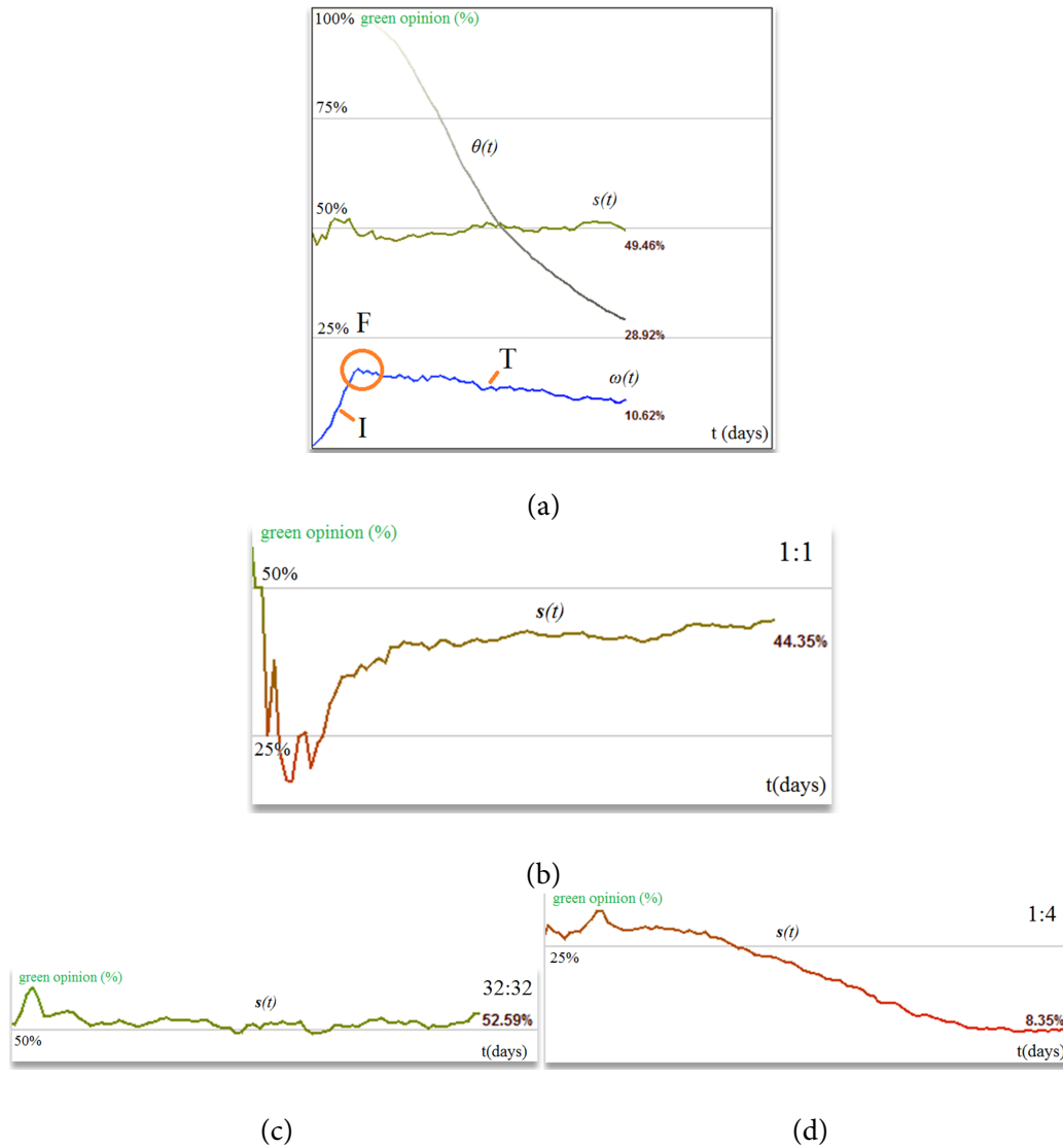
Figure 6.10.: Simulation of a 100,000 mesh network with SocialSim [253], displaying a representative example for the evolution of s(t) , \theta(t) , and \omega(t) , as well as the opinion evolution s(t) with various stubborn agents distributions. a. Mesh topology, where the lowest panel displays the opinion change ( \omega ) evolution over three simulation phases. b. Opinion evolution s(t) with few and evenly distributed SA (1:1 ratio: 1 green, 1 red). c. Opinion evolution with many and evenly distributed stubborn agents (1:1 ratio: 32 green, 32 red), d. Opinion evolution with few and unevenly distributed stubborn agents (1:4 ratio: 1 green, 4 red).
