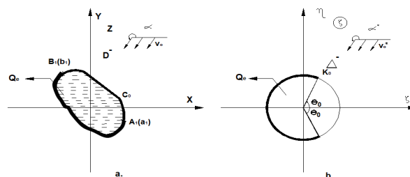
Figure 2. Scheme of conformal mapping of the flow domain in the complex plane ( z ) on the external domain of a circle in the complex plan ( \zeta )
