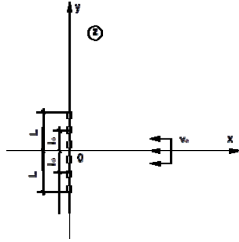
Figure 3. Scheme of drainage trench disposed in a parallel groundwater flow
