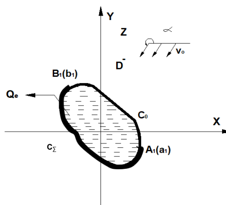
Figure 1. Scheme of a recharge/discharge cavity in shallow aquifer (plan view)
