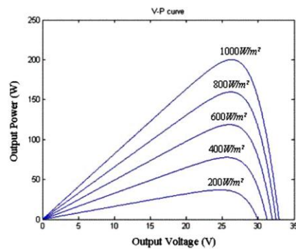
Fig.3. V-P Characteristics of Solar cell
