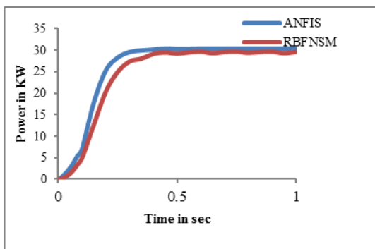
Fig.10. MPPT Performance of WECS
