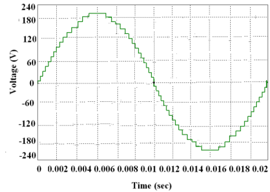
Figure 6 .31 level output voltage by NR method
