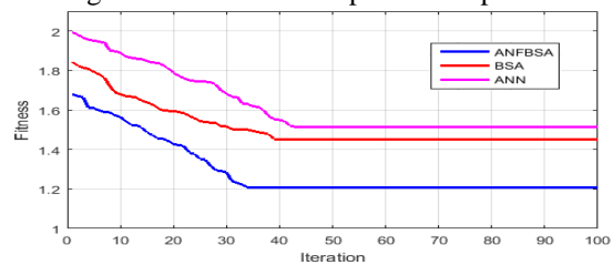
Fig. 12. Fitness comparison
