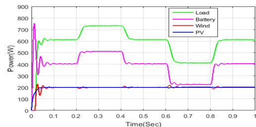
Fig. 11. Total resources power comparison
