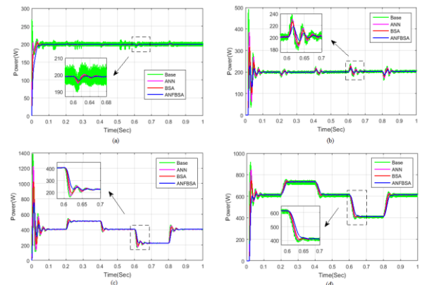
Fig 10: Comparison analysis of (a) PV (b) Wind (c) Battery (d) Load
