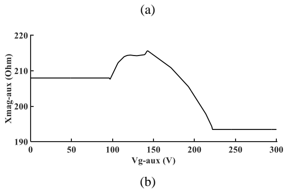
Fig.5 The magnetization characteristic for (a) main winding and (b) auxiliary winding
