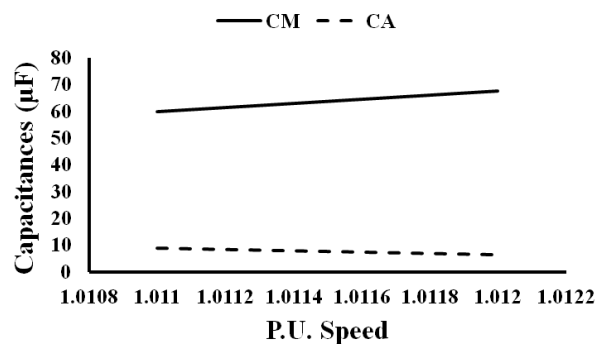
Fig.12 Main and Auxiliary capacitance versus P.U. speed at a load of 185 ohm and 0.65 power factor
