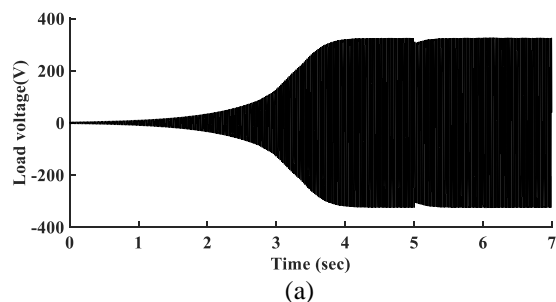
Fig.13 No-Load building up process (a) main winding voltage, (b) auxiliary winding voltage (c) main winding current, (d) auxiliary winding current (e) main winding magnetizing inductance, (f) auxiliary winding magnetizing inductance and (g) main winding frequency
