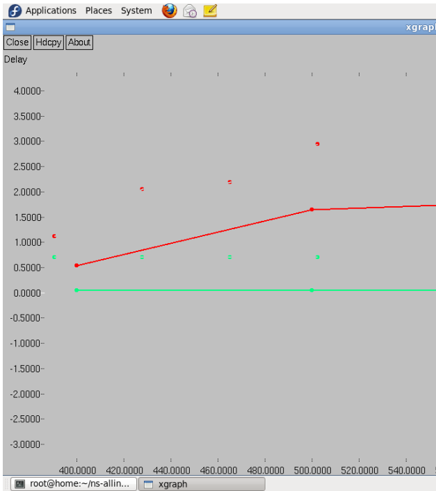
Figure 4 represents the Packet size 400 delay is 0.5 seconds, 500 packets the delay is 1.5seconds ,600 packets the delay is 1.8seconds and finally for 700 packets the delay is 2.5seconds in DAPP scheme if packet size increases the delay is increased. But in the EAFWFQ the packet size 400 delay is 0 seconds delay,500 packets size - 0.1 microseconds,600 packet size- 0.15microseconds,for packet size 600 the delay is -0.18microseconds,for packet size 700 the delay is -0.5 microseconds. By Comparing DAPP scheme and EAFWFQ scheme , delay is much less in our proposed scheme.
