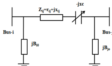
Fig.2 Location of TCSC in the transmission line
