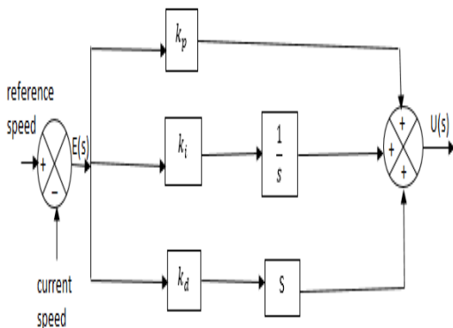
Figure. 2 Block diagram of PID controller
