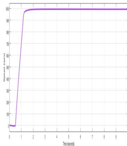
Figure.11. Speed response due to FOPID controller
