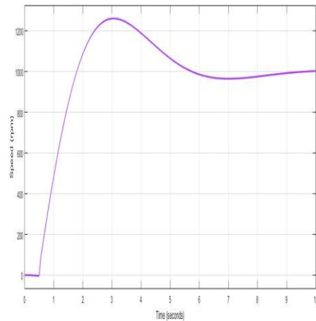
Figure. 10 speed response due to PID controller
