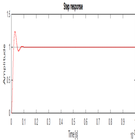
Figure. 9. PID step response by genetic algorithm
