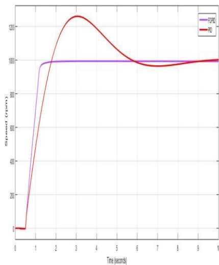
Figure. 12. Comparison of PID and FOPID speed response.
