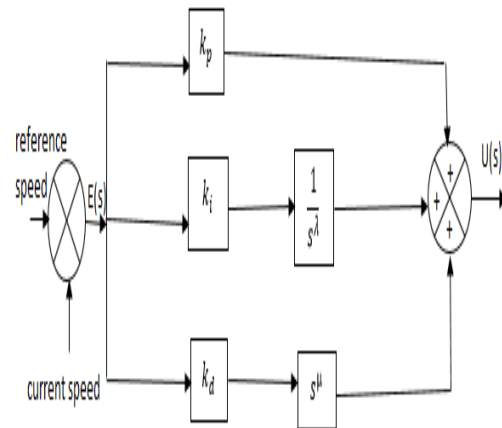
Figure. 3. Block diagram of FOPID controller
