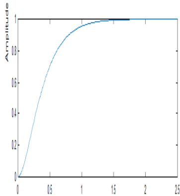
Figure.8. FOPID step response by genetic algorithm
