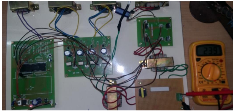
Fig. Experimental Setup for IDVR
