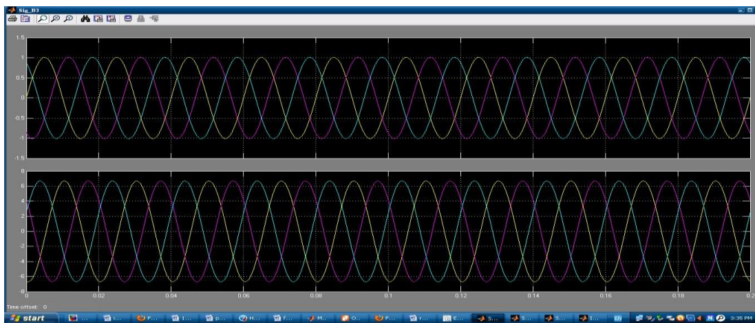
Fig.5.The stabilized output response (V load; I load) when IDVR is added in the model
