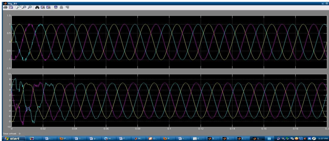
Fig 4. The output response (V load; I load) of the model when the IDVR is not added
