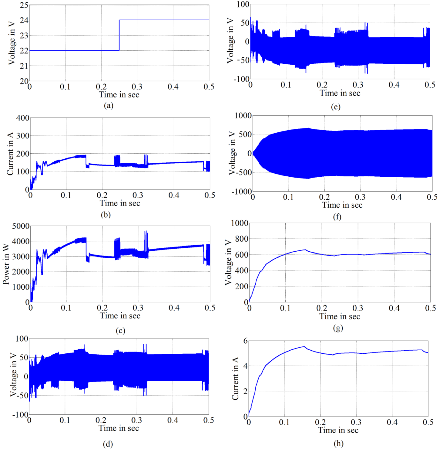
Figure 7. Case 1 Simulation Results: (a) PV array voltage; (b) PV array current; (c) PV Power; (d) Primary 1 Voltage; (e) Primary 2 Voltage; (f) Secondary Voltage; (g) DC Link Voltage; (h) DC link Current.
