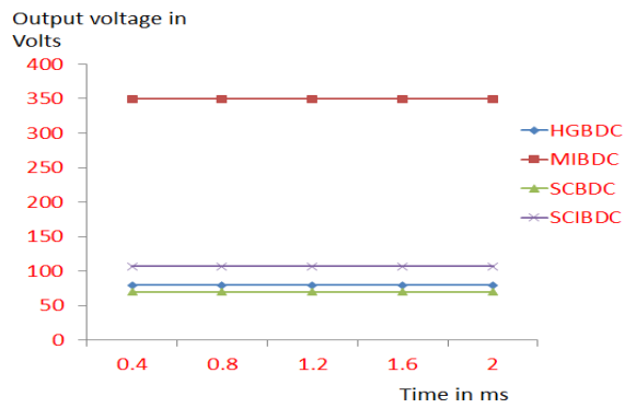
Fig. 5. Output voltage for different Bidirectional DC-DC Converter topologies
