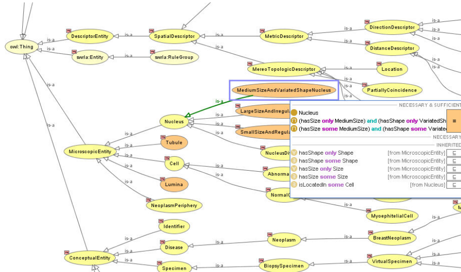
Figure 7.3. Fragment of the inferred model of ontology- OWLViz view
