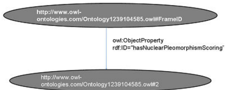
Figure 7.5. RDF representation
