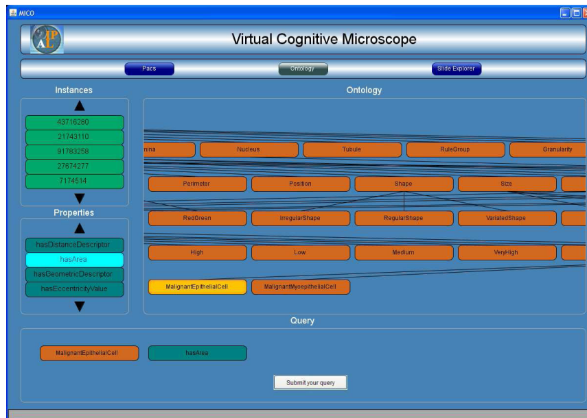
Figure 8.8. Ontology management
