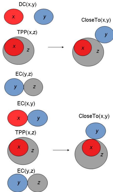
Figure 5.4. CloseTo relation
