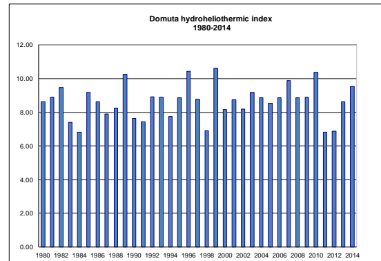
Figure 8. Domuta hydroheliothermic index.
